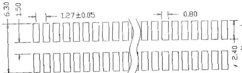
P. C. B LAYOUT
